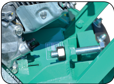
EZ-Set cutter depth adjuster.
