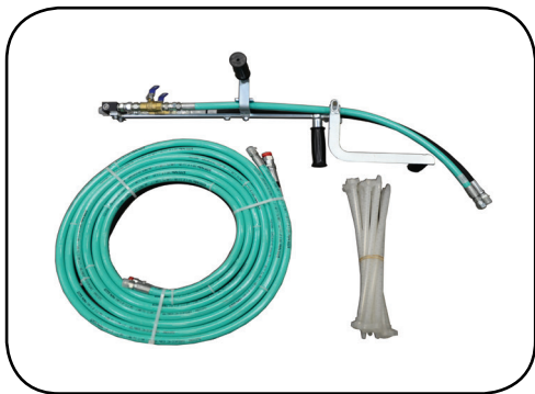
Robust operator wand assy. with dual hose. Products mixed at tip for easy clean up.
